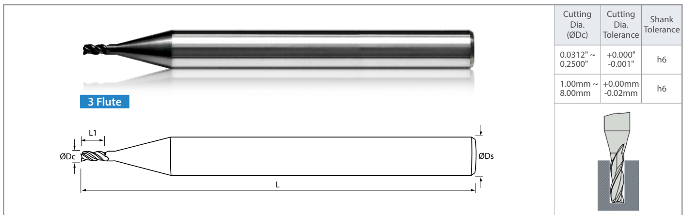
Inch Size Dimensions
