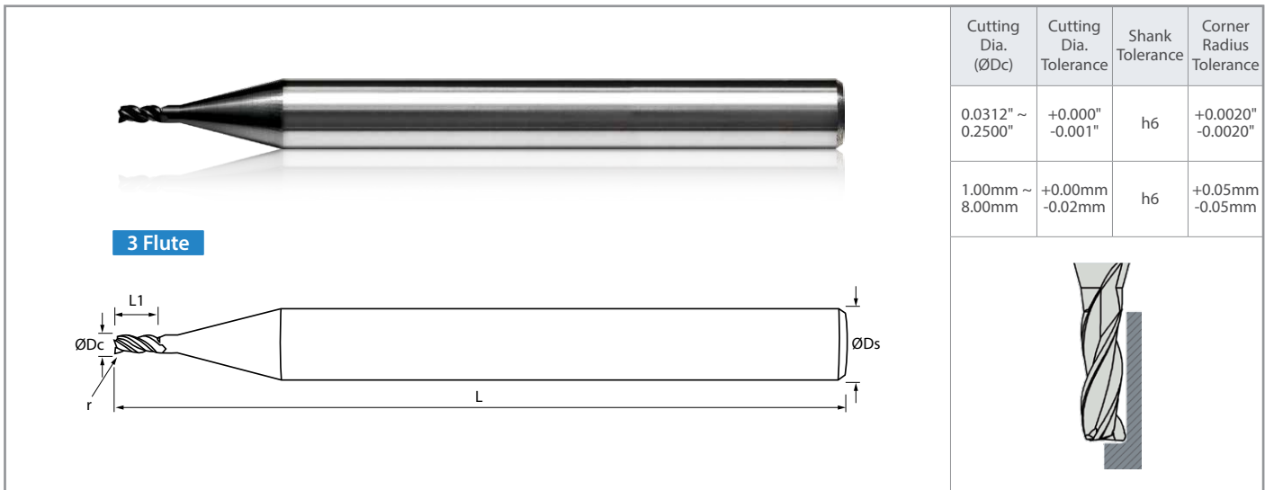
Inch Size Dimensions
