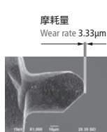
切削後 After machining
