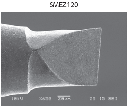
CBNマイクロエッジZ特殊刃形状 CBN Micro Edge Z original flute design.
