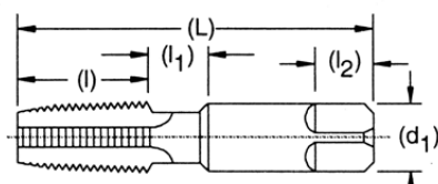
Tap Dimensions - Inches
